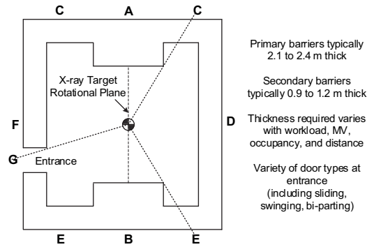
Figure 2-3 Simplified drawing of treatment room with no maze.
