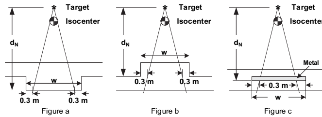
Figure 2-6 Primary barrier width.
