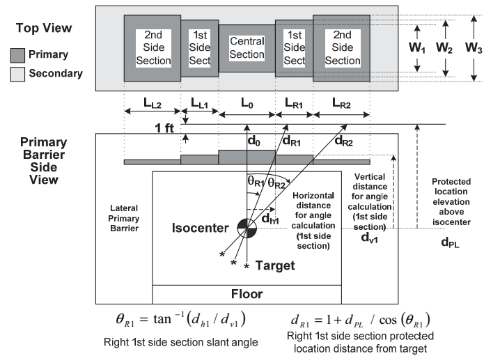
Figure 2-9 Tapered primary ceiling barrier.
