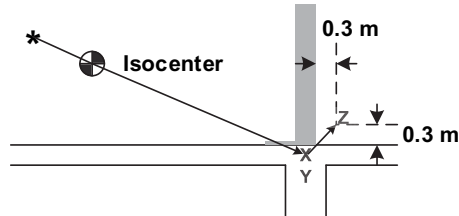
Figure 2-10 Basic groundshine geometry.
