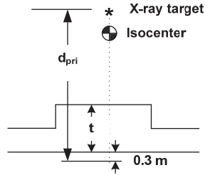
Figure 2-4 Primary barrier geometry.
