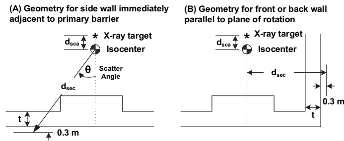
Figure 2-5 Secondary barrier geometry.
