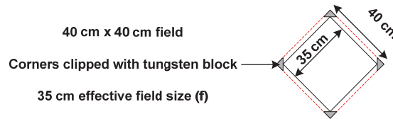
Figure 2-7 Effective field size.
