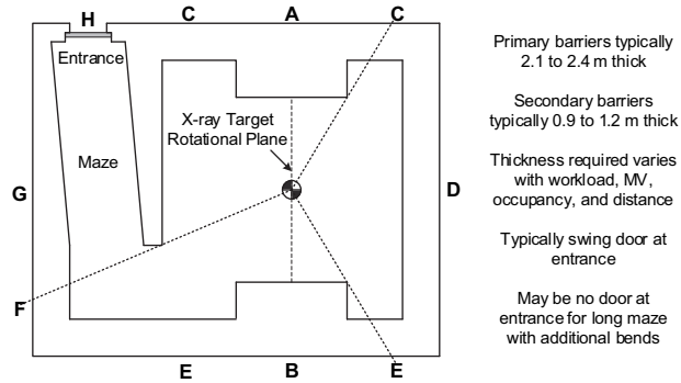
Figure 2-1 Simplified drawing of treatment room with maze. (Letters in the figure are referred to in the text.)
