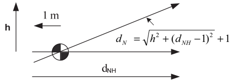
Figure 2-8 Distance measured to top of primary barrier.
